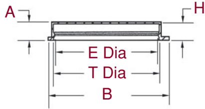
Snap Closure
